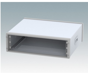
M6019325 INSTRUMET 19" 3Ux450mm Aluminium Light grey/window grey RAL 7035/7040 157x516x450mm
