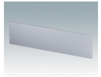
M6019001 Front panel 3Ux19" Aluminium Matt anodised 482.6x3x132.5mm
