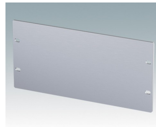
M6010001 Front panel 3Ux10.5" Aluminium Matt anodised 269.2x3x132.5mm
