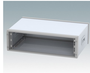
M6019305 INSTRUMET 19" 3Ux350mm Aluminium Light grey/window grey RAL 7035/7040 157x516x350mm
