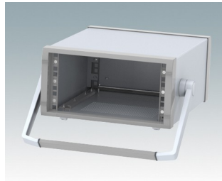
M6010315 INSTRUMET 10.5" 3Ux350mm Aluminium Light grey/window grey RAL 7035/7040 157x303x350mm
