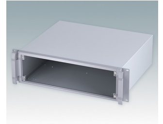
M5619335 UNIMET 19" 3Ux380mm Aluminium Light grey/window grey RAL 7035/7040 132.5x482.6x380mm
